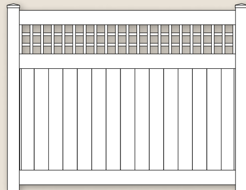
V32150E Privacy Fence with Old English Lattice Top (All rails are 2" x 6". Old English Lattice features 7/8" x 1-1/2" Pickets Crossing Through 1-1/2" x 1-1/2" Pickets)
