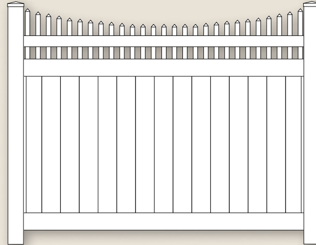
V3707 Tongue and Groove Privacy Fence with Scalloped Classic Victorian Picket Top
